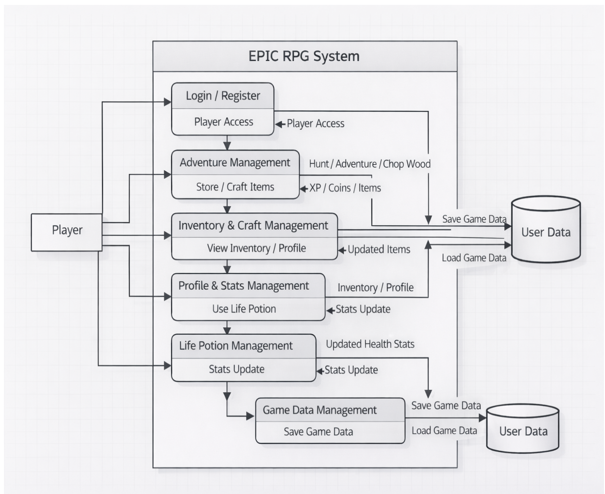
Figure 5.3 DFD Level-1
